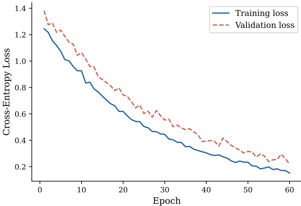
FusionNet Training Convergence
