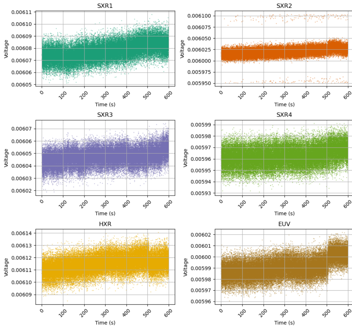
Figure 1: Raw voltage vs. time (s) for all six ASIO channels.
