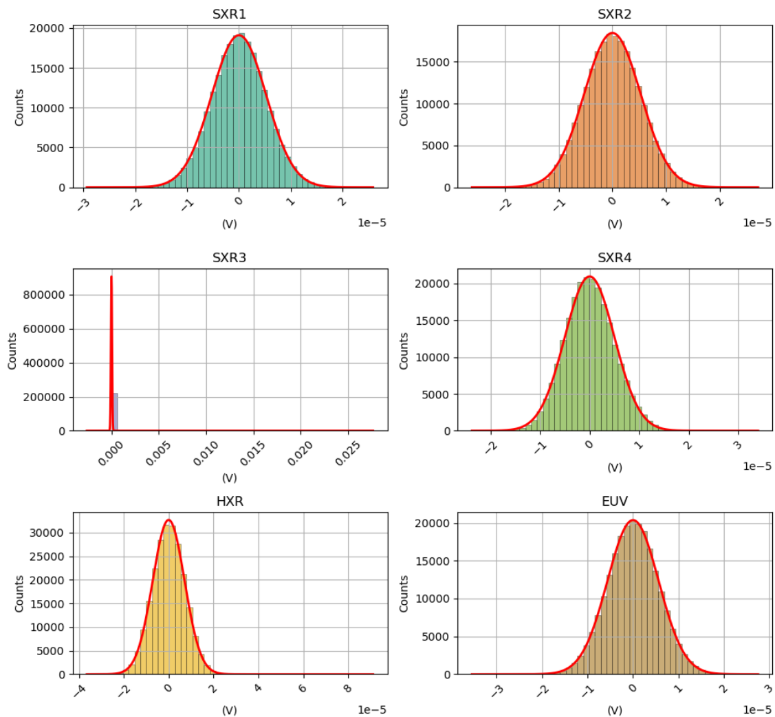
Figure 4: Noise histograms after detrending and 40 Hz EMI removal. Red curve is a Gaussian fit.
