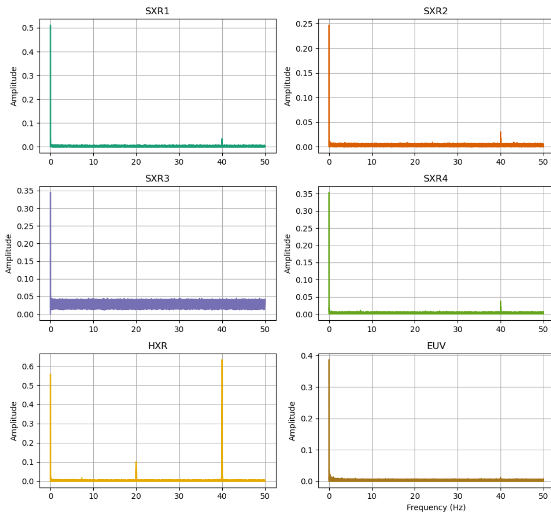
Figure 2: FFTs of raw voltages (mean centered).
