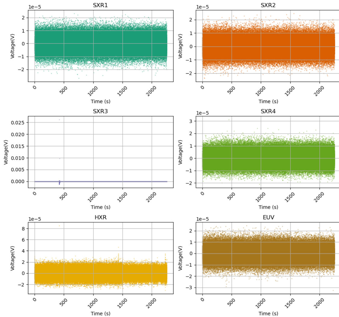
Figure 3: Voltage vs. time (s) after Savitzky–Golay detrending and 40 Hz EMI removal.
