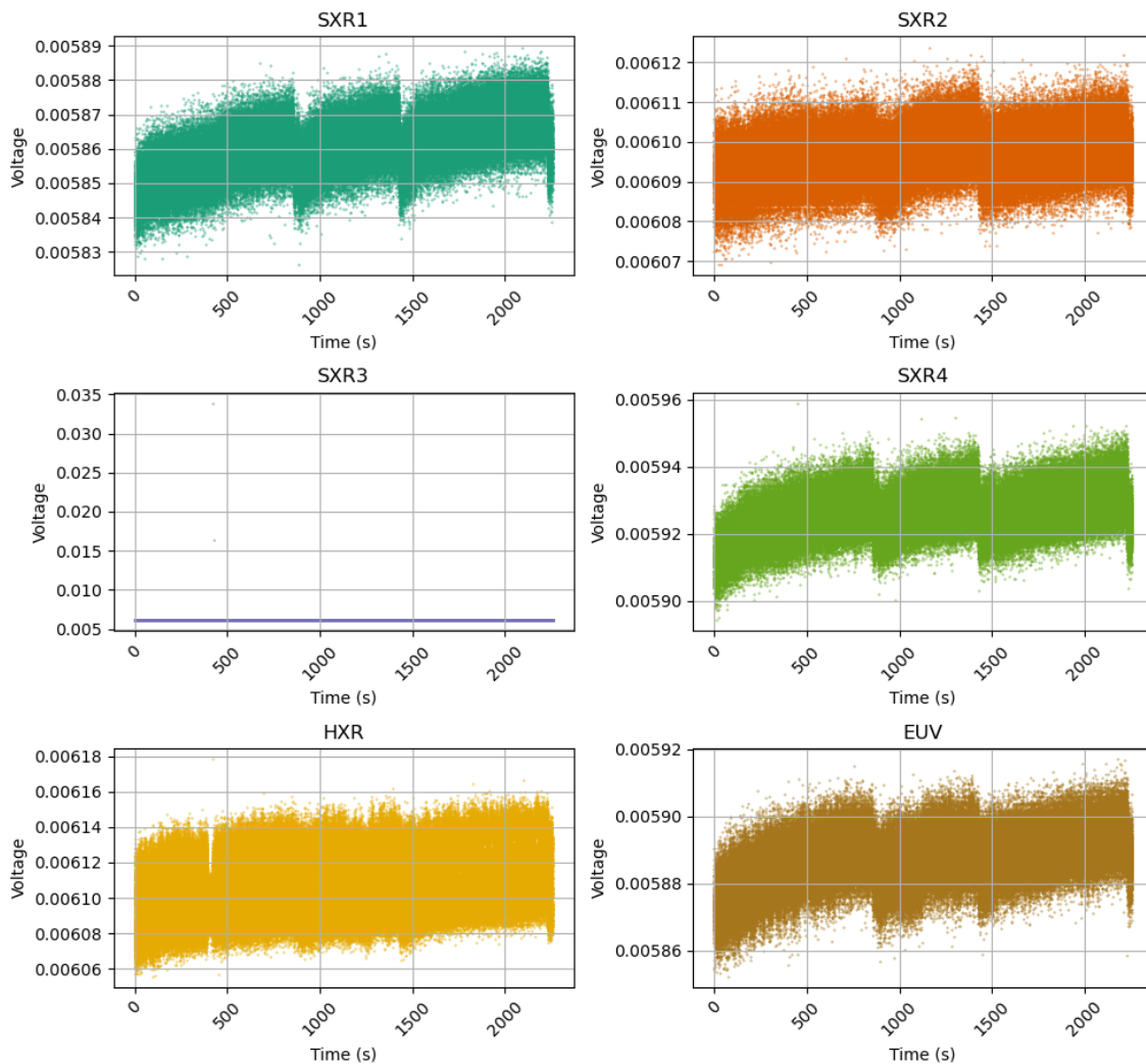
Figure 1: Raw voltage vs. time (s) for all six ASIO channels.
