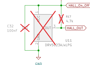
Hall-effect sensor
