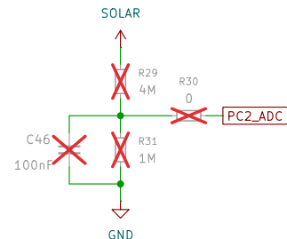
Onboard solar voltage sensing
