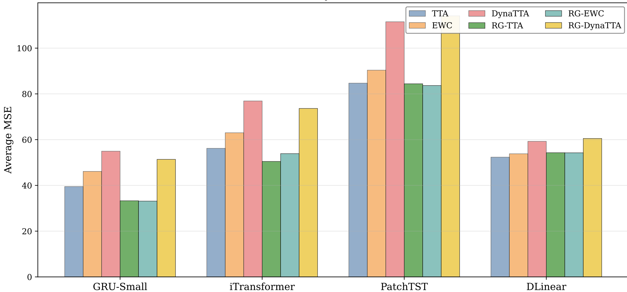
Real-World MSE by Model Architecture
