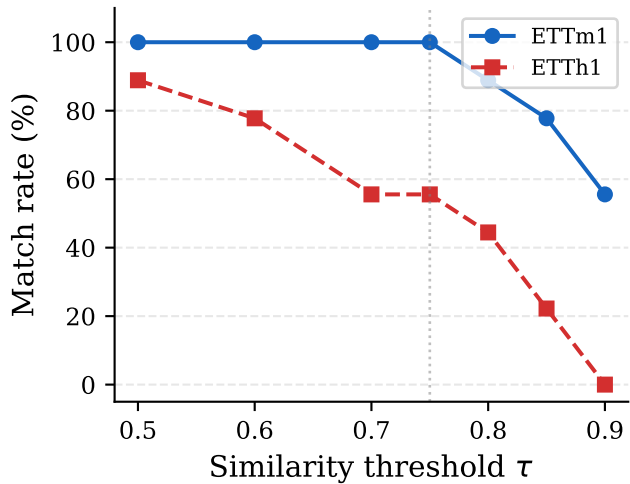
(b) Checkpoint reuse vs. \tau threshold
