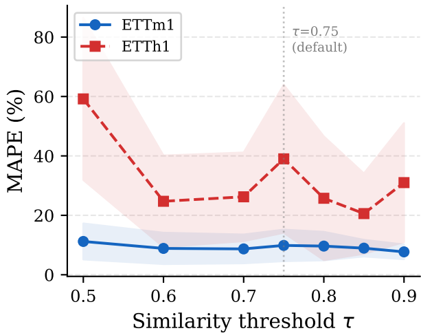
(a) Accuracy vs. \tau threshold
