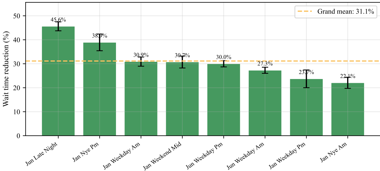
Per-scenario improvement (Cal+LP vs Replay, 5 seeds, 95% CI)
