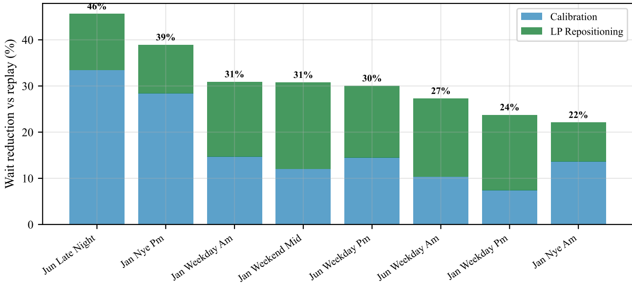
Component decomposition: Calibration + LP contributions
