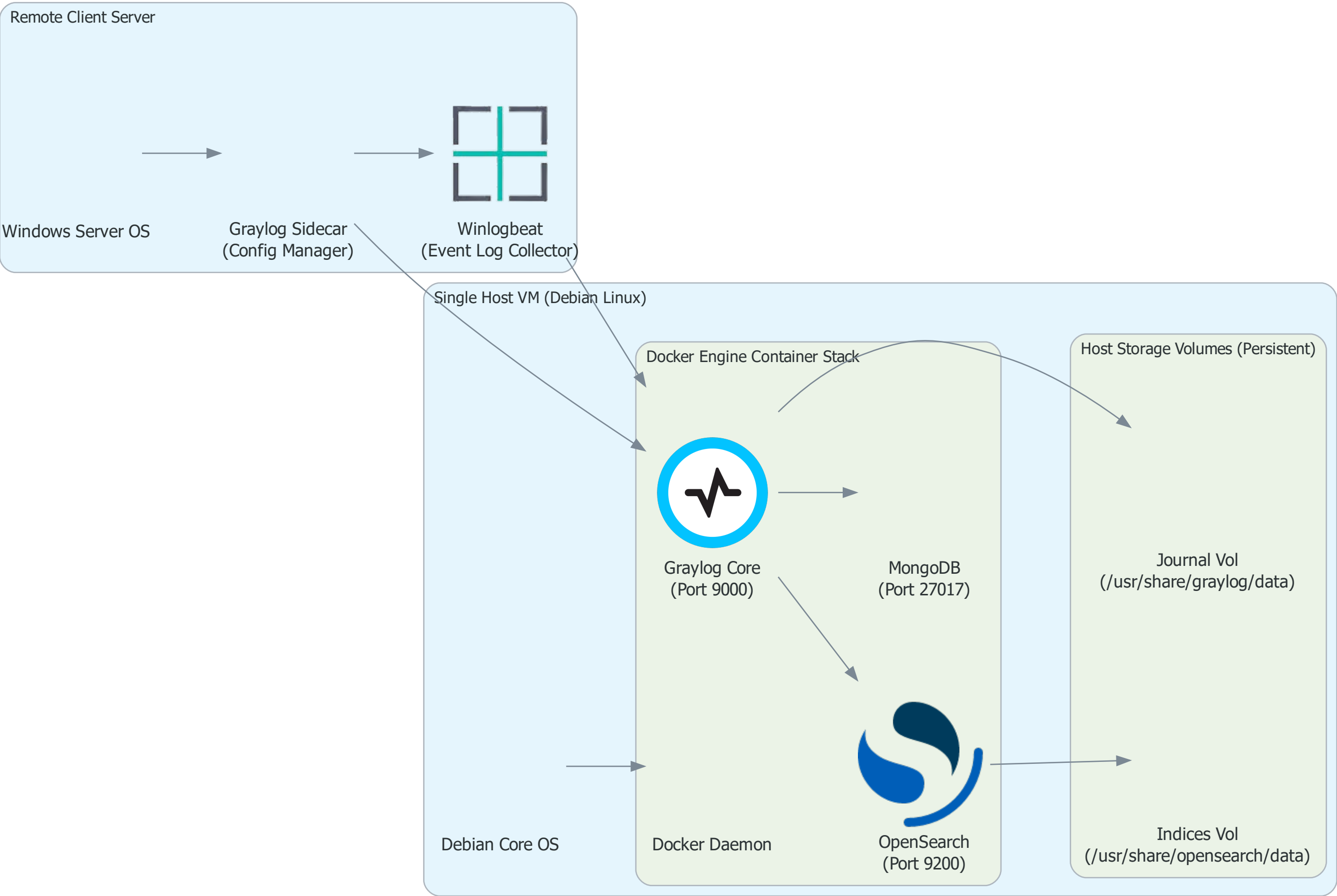
Graylog Single Node Architecture
