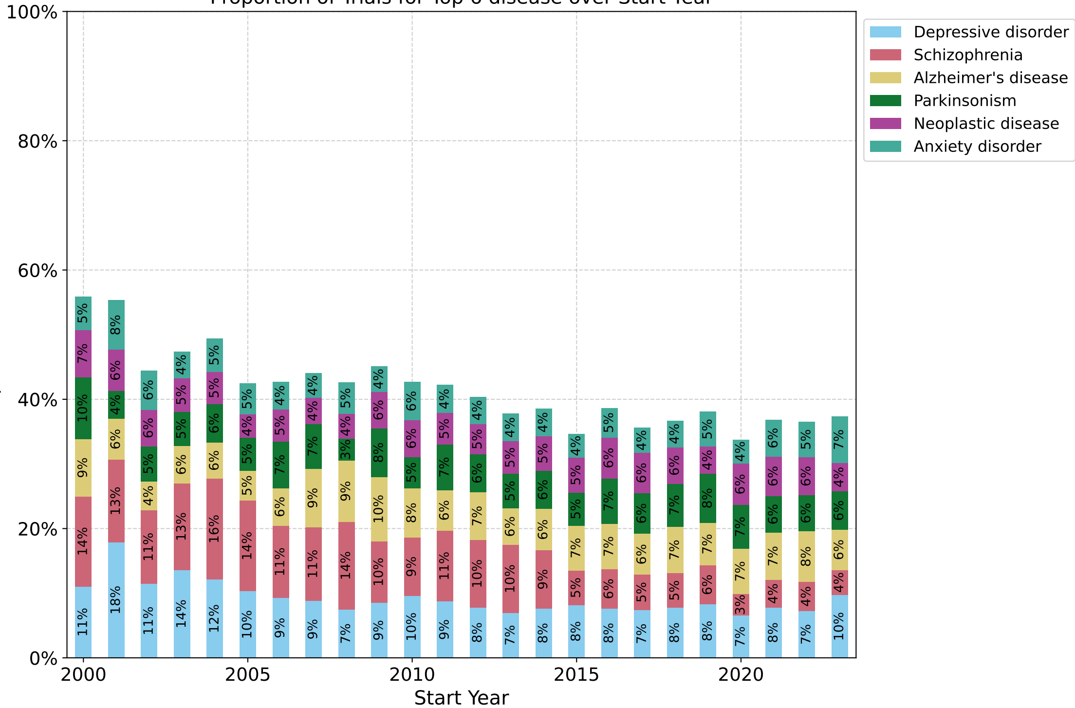
Proportion of Trials for Top 6 disease over Start Year
