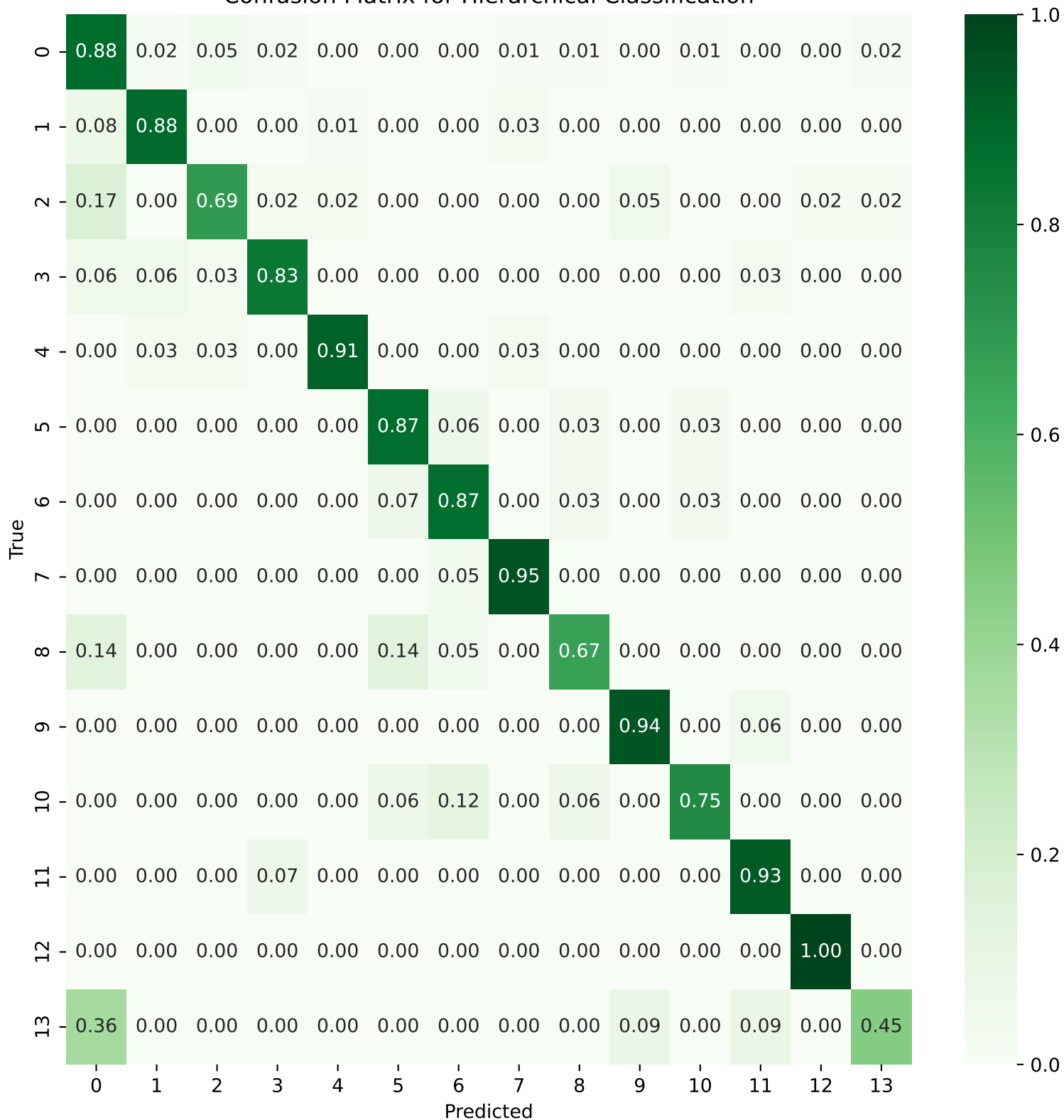
Confusion Matrix for Hierarchical Classification
