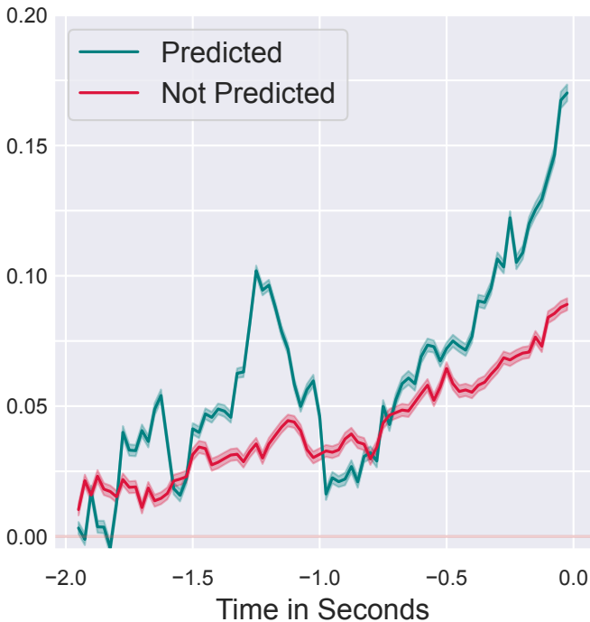
Cross-validated Correlation
