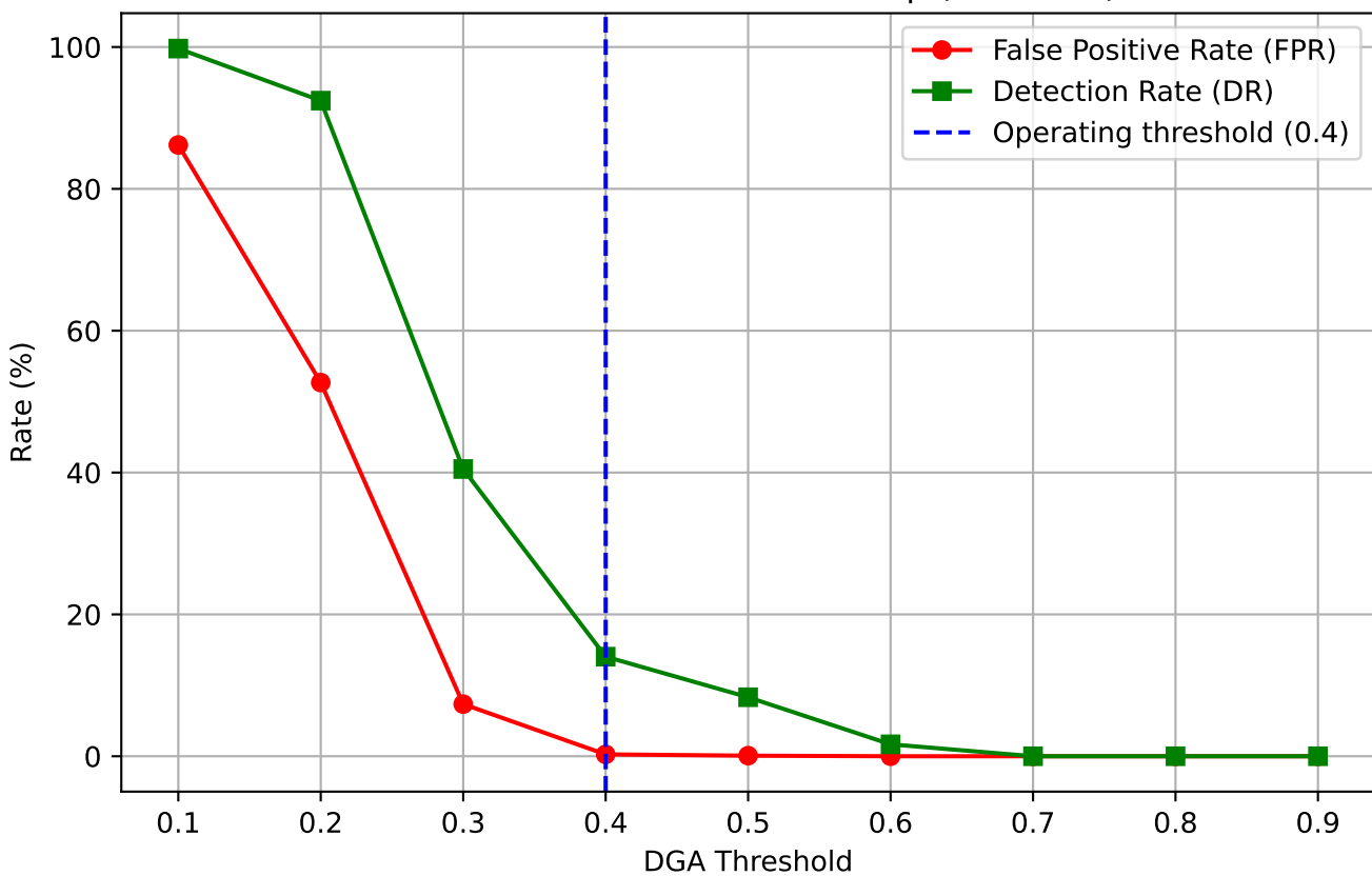
DGA Detection Threshold Sweep (UMUDGA)
