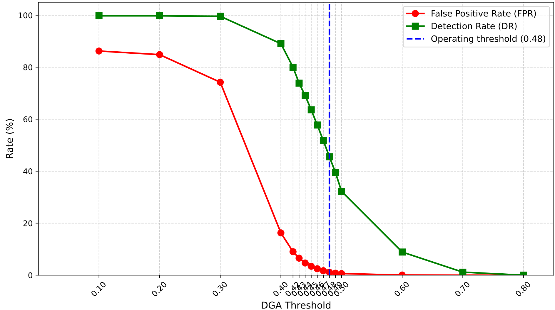
DGA Detection Threshold Sweep (Improved 4-gram Scorer)
