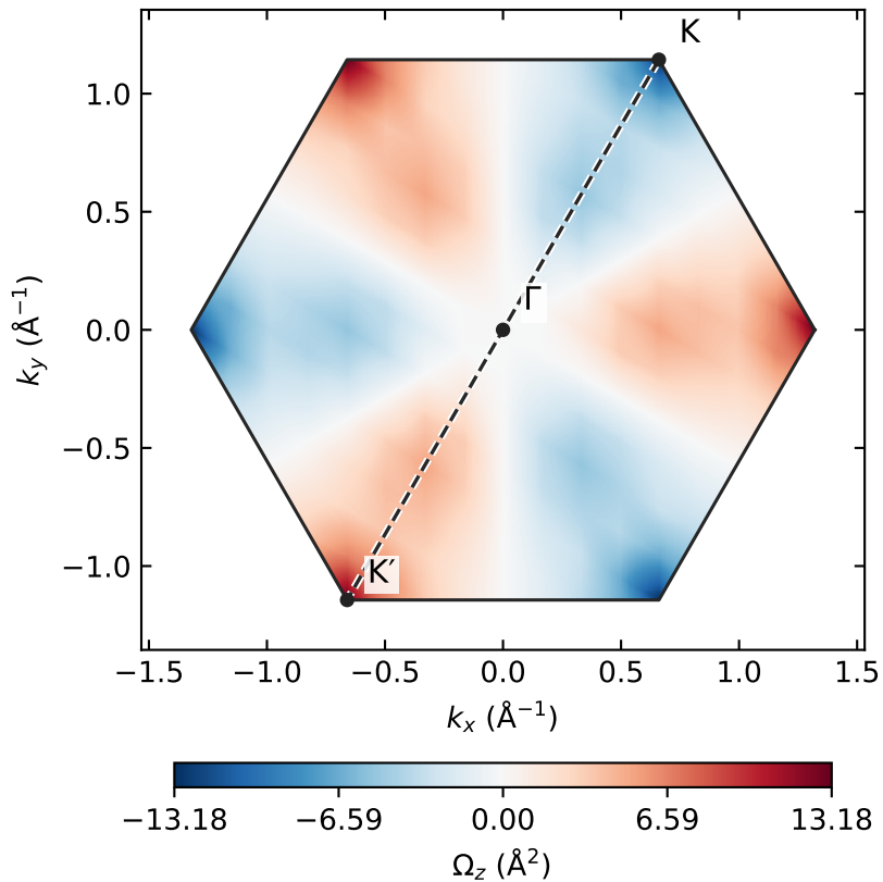
(a) Kubo: occupied bands 1-18
