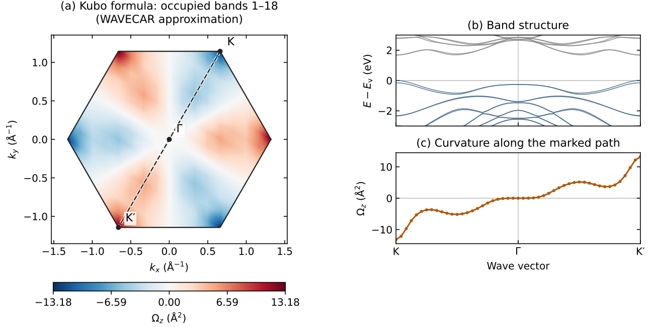
Figure 2. (a) Canonical-momentum Kubo trace curvature of occupied bands 1–18 on the 12 \times 12 mesh. Only transitions to the stored empty bands 19–26 enter the sum. The map uses the same periodic bilinear display interpolation and dashed K– \Gamma –K' path as Figure 1. (b) VASP band structure, with occupied bands in blue and empty bands in gray. (c) Bundle curvature calculated directly at all 49 path points. Internal valence-band degeneracies do not interrupt the bundle curve.
