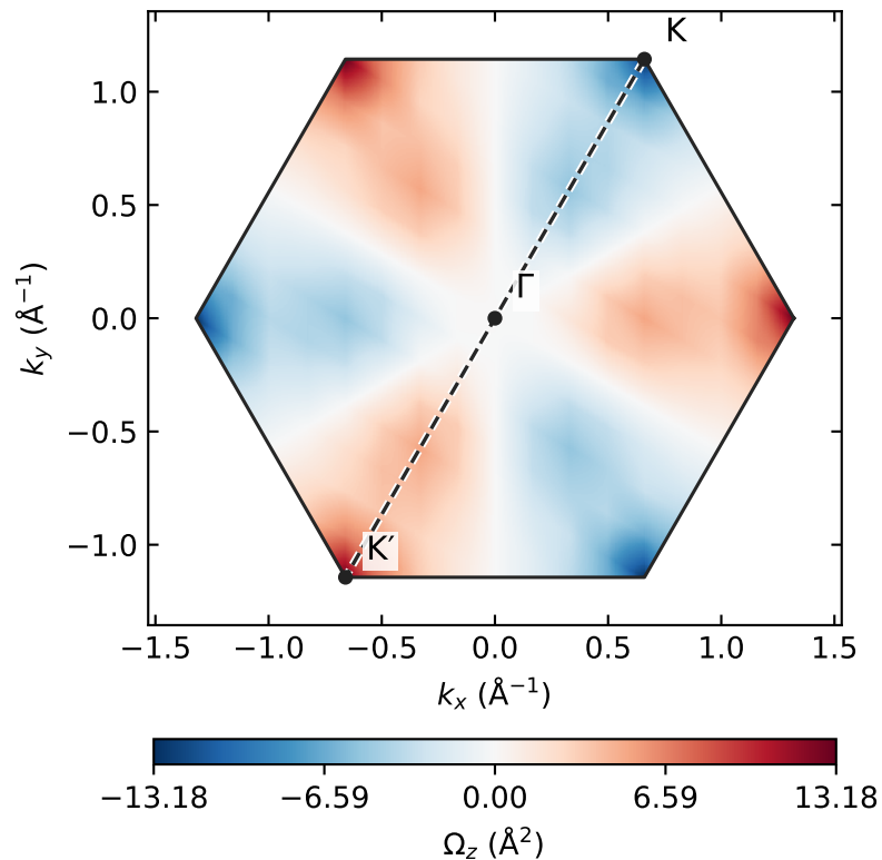
(a) Kubo formula: occupied bands 1-18 (WAVECAR approximation)
