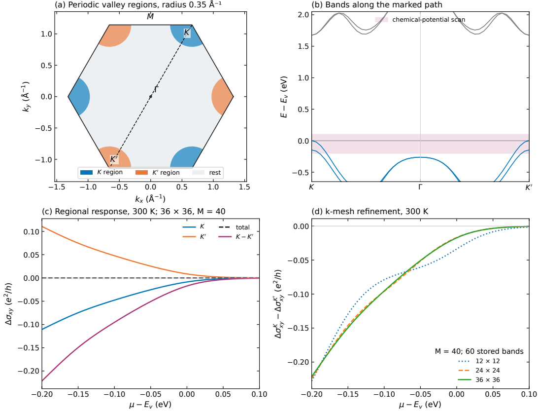
Figure 4. (a) Cartesian first BZ with periodic K/K' disks of radius 0.35 \text{ \AA}^{-1} and the marked K-Γ-K' line. (b) The matching 26-band VASP dispersion, with the chemical-potential interval shaded. (c) Regional Hall changes at 300 K on the 36 \times 36 mesh, using 60 stored bands and pairs within bands 1–40. (d) Mesh refinement at that fixed band window. Energies are relative to each source's valence-band maximum; the band path uses the same density and cutoff.
