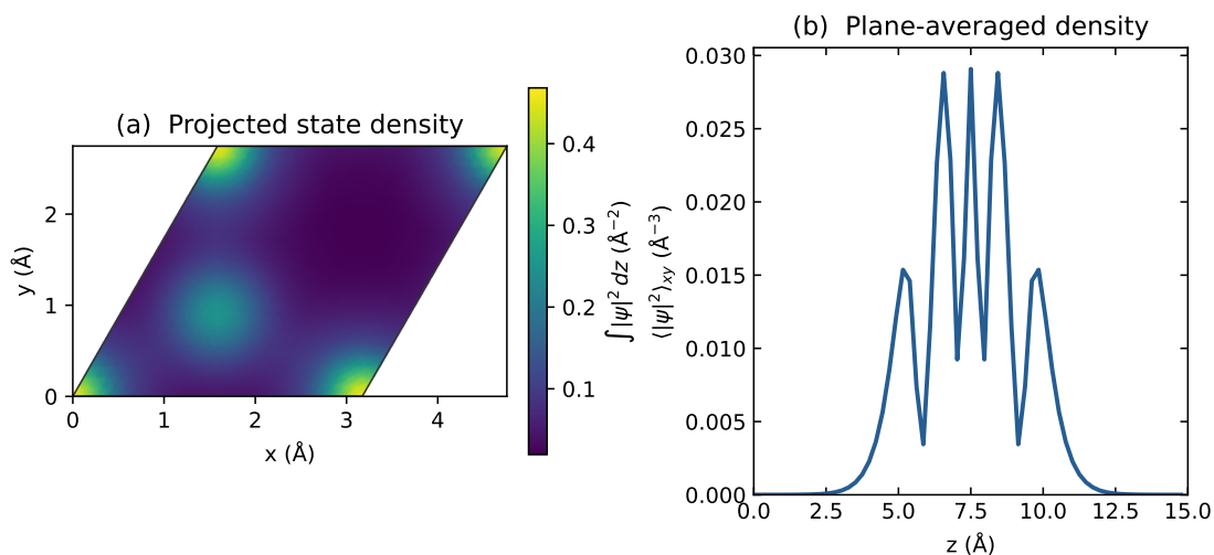
Figure 9. Projected pseudo-wavefunction density of band 18 at \Gamma and its plane average along z . The in-plane plot uses the Cartesian geometry of the oblique primitive cell. Both spinor components are retained.
