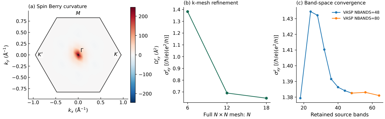
Figure 8. (a) Occupied-bundle spin Berry curvature \Omega_{xy}^z , from PAW spin and full velocity matrices on the 12 \times 12 VASP mesh, shown in the Cartesian first BZ. Periodic bilinear interpolation is used only for the color map. (b) Mesh refinement retaining 48 bands from 64-band VASP sources. (c) Retained-band studies from 48- and 80-band VASP sources at a fixed 6 \times 6 mesh. The numerical integrals always use the original k points and weights.
