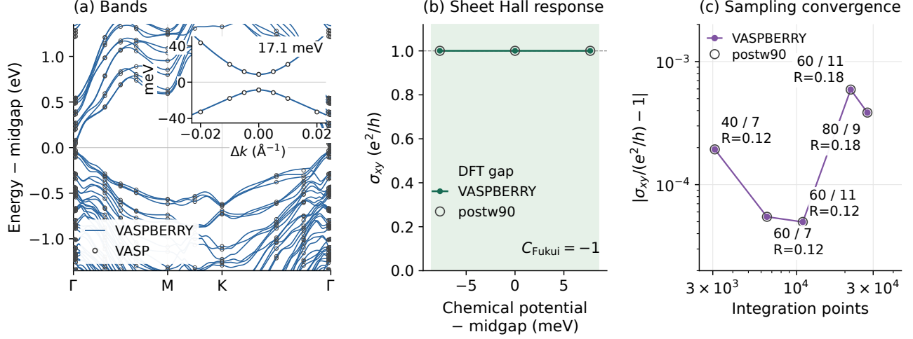
Figure 10. (a) VASPBERRY-interpolated bands along \Gamma -M-K- \Gamma , with direct VASP checks; the inset resolves the K- \Gamma -M gap near \Gamma . (b) VASPBERRY full-connection sheet Hall response at three chemical potentials inside the gap, at zero temperature; open markers show the independent postw90 comparison. The dashed line is the topological expectation. (c) Deviation |\sigma_{xy}/(e^2/h) - 1| under integration refinement. Labels give the base mesh, local subdivision and \Gamma -region radius in \text{\AA}^{-1} . Both solvers use the same model and weights; their agreement is distinct from mesh convergence.
