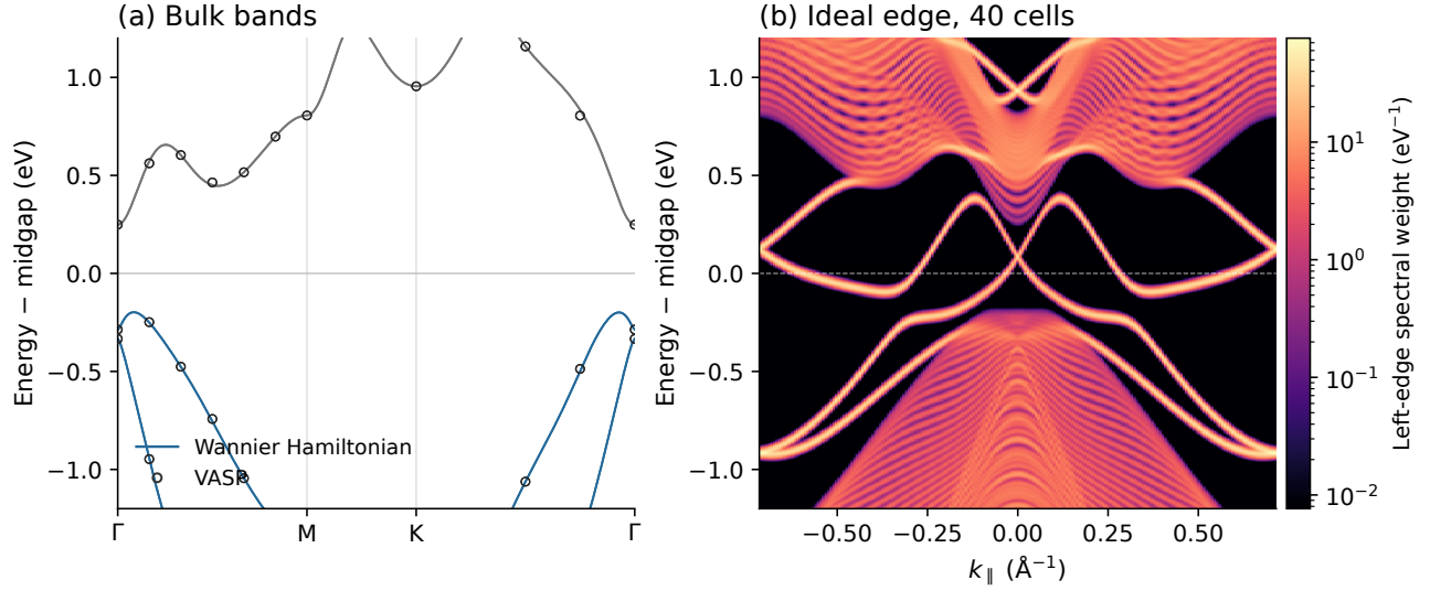
Figure 7. (a) VASPBERRY bands from the VASP-derived 16-orbital Wannier Hamiltonian along \Gamma -M-K- \Gamma . Circles show direct VASP energies on the independent 12 \times 12 mesh; all ten occupied bands are retained in the model. (b) Spectral weight in the first two cells of a 40-cell strip, periodic along the first lattice vector and open along the second. All eigenstates are summed before applying a 10 meV Gaussian display broadening. Energy zero is the midpoint of the sampled VASP bulk gap. The edge branches connect the valence and conduction manifolds across that gap.
