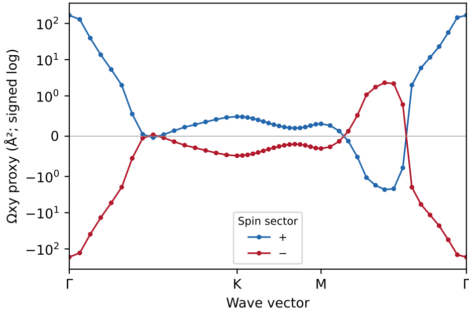
(a) Occupied path bands 1:10
