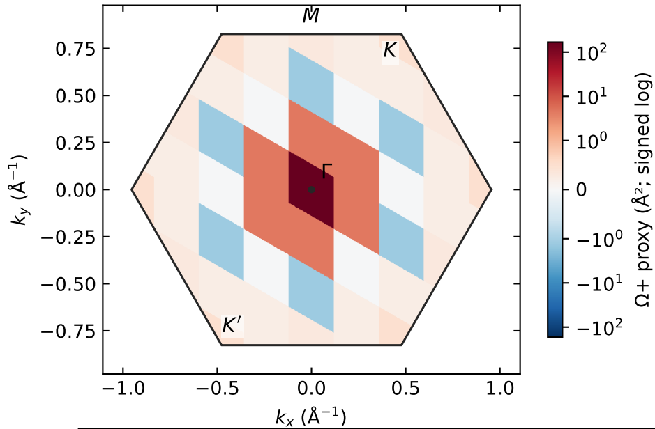
(c) Occupied full-BZ point samples
