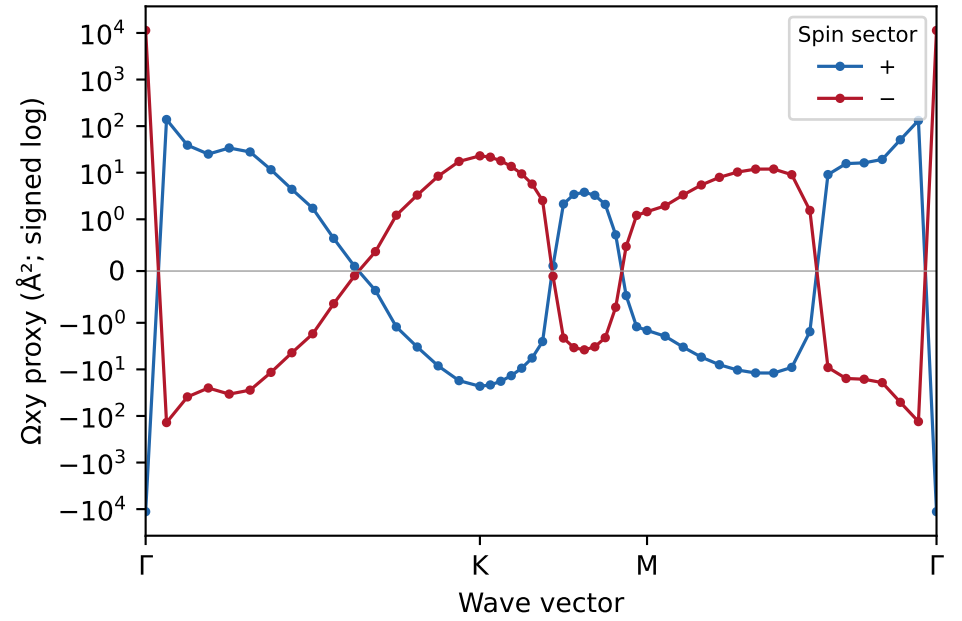
(b) Selected pair path bands 9:10
