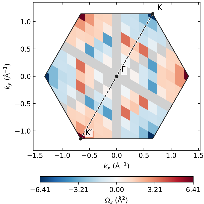
(a) Kubo: band 18
