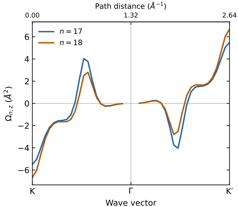
(b) Berry curvature
