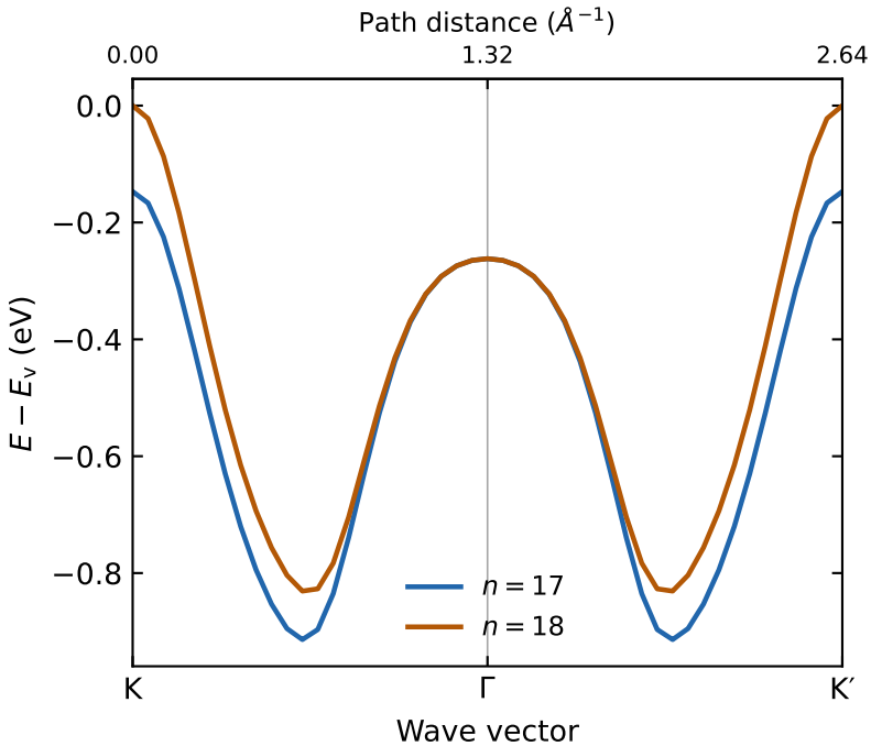
(a) Valence-band dispersion
