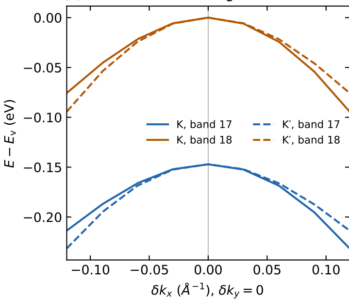
(c) Valence bands along the dashed cuts
