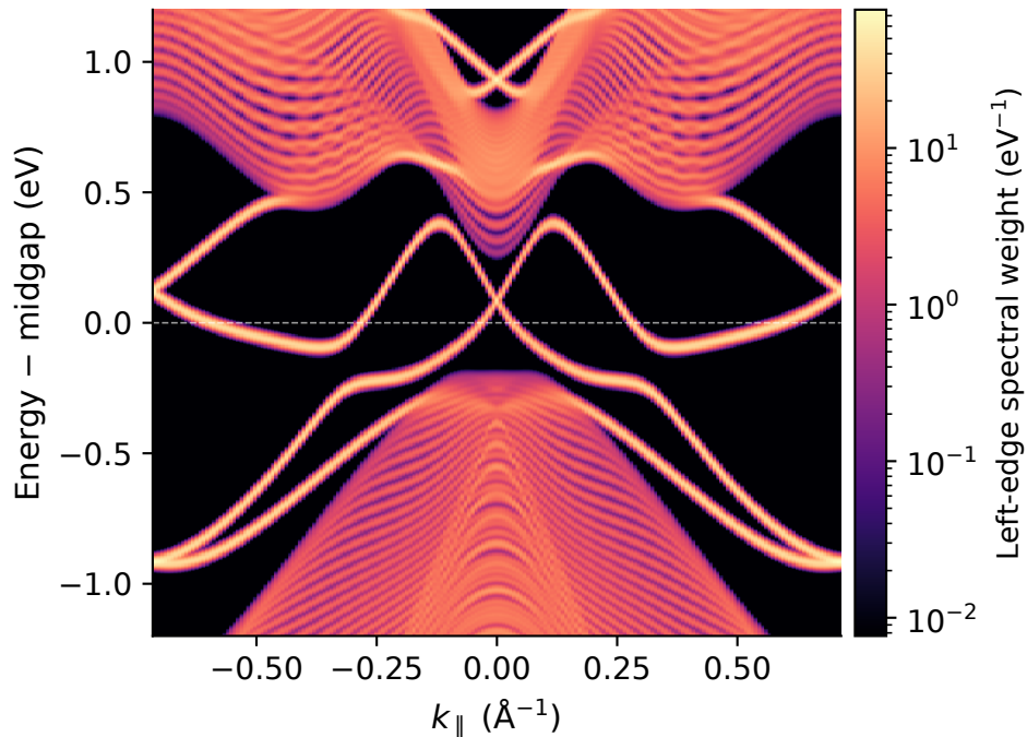
(b) Edge check of Z_2 = 1 , 40 cells
