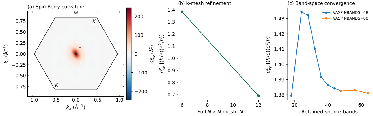
Figure 8. (a) Occupied-bundle spin Berry curvature \Omega_{xy}^z from PAW spin and full velocity matrices on the 12 \times 12 VASP mesh, shown in the Cartesian first BZ. Periodic bilinear interpolation is used only for the color map. (b) Mesh refinement retaining 48 bands from 64-band VASP sources. (c) Retained-band studies from 48- and 80-band VASP sources at a fixed 6 \times 6 mesh. The numerical integrals always use the original k points and weights.
