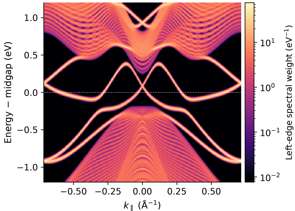
(b) Ideal edge, 40 cells
