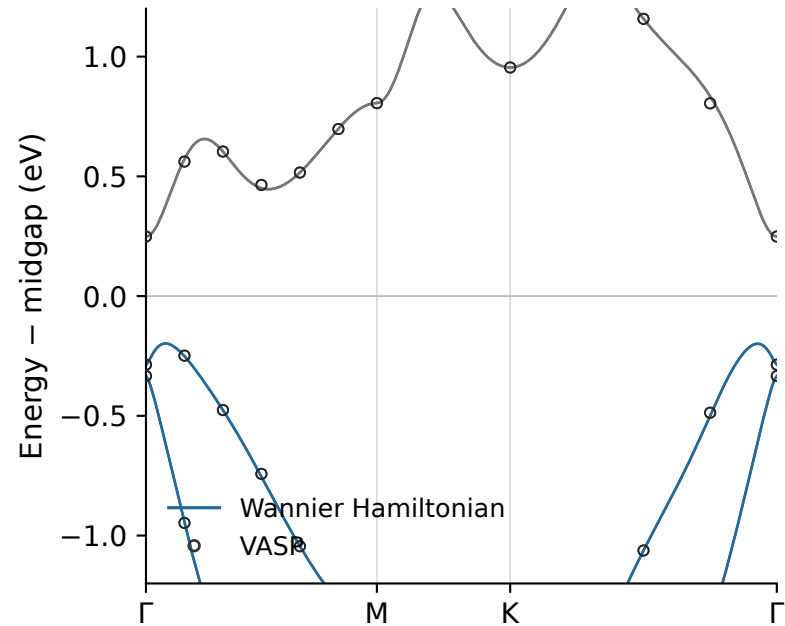
(a) Bulk bands
