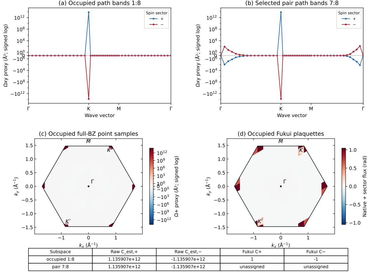
Figure 10. (a) Positive/negative occupied-sector Kubo curvature along \Gamma -K-M- \Gamma . (b) Local curvature of the 7-8 pair, without a global Chern assignment. (c) Raw occupied positive-sector point curvature on the 12 \times 12 mesh. (d) Independent positive-sector Fukui plaquette flux. Signed-log display exposes both signs and the very large peaks; it does not modify the stored data or repair the mesh integral. The example plotter reads native CSVs, changes no wavefunctions and performs no additional curvature calculation. Reference data and input/output hashes accompany the figure.
