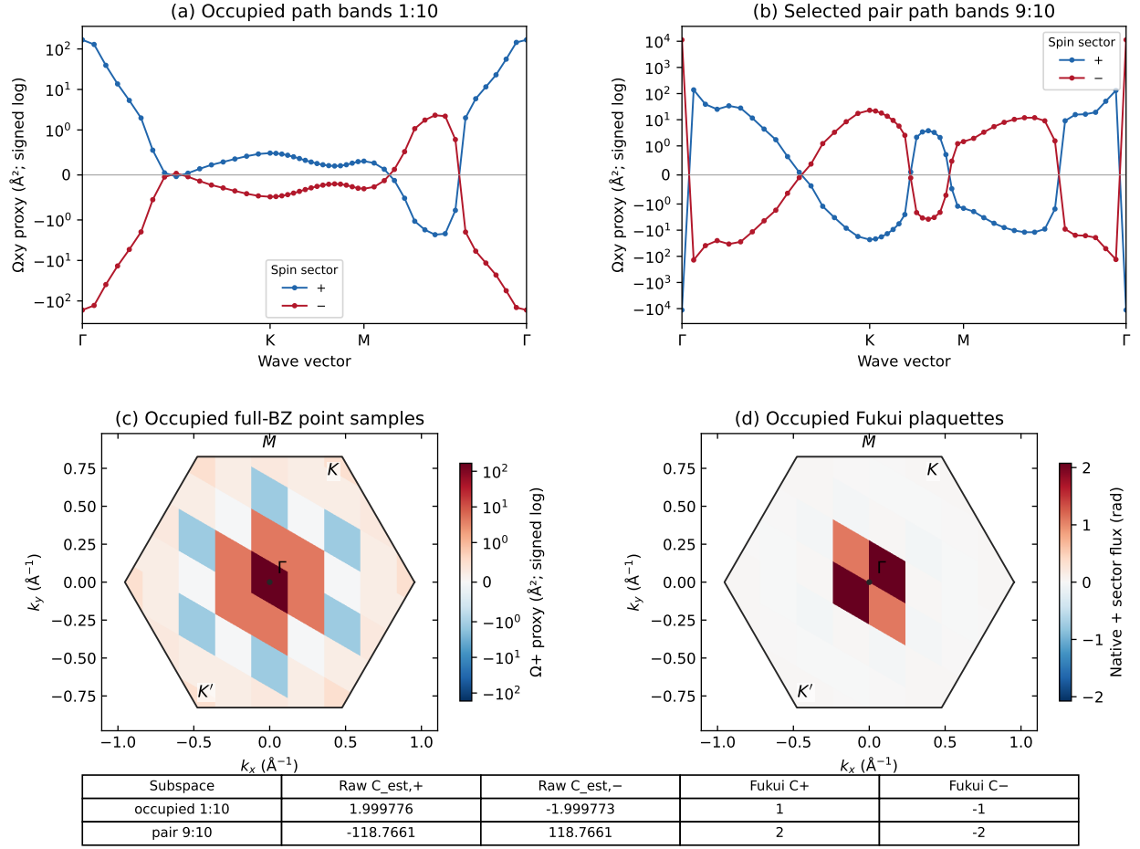
Figure 11. (a,b) Actual 49-point occupied and pair-sector path curves. (c) Occupied positive-sector point curvature on the 6×6 mesh. (d) The same occupied space’s independent positive-sector Fukui flux. All panels use native outputs. Straight segments connect path samples only; no interpolated Hamiltonian supplies extra samples. The saved decomposition columns permit additional plots of the parent contribution and the projected-spin mixing correction.
