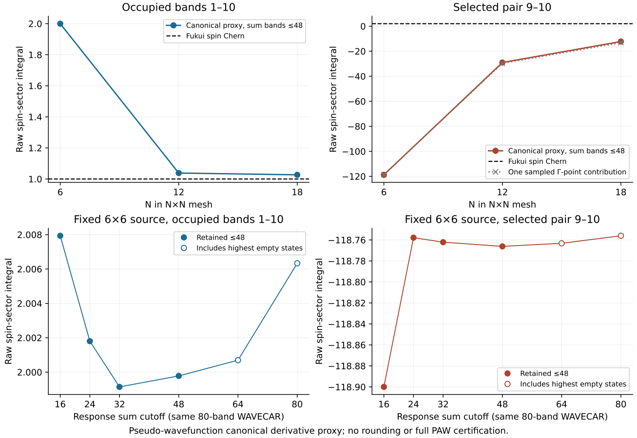
Figure 12. Bi mesh and intermediate-state controls using the same Hamiltonian. The figure retains noninteger and negative raw estimates; Fukui values are shown as independent geometric references. The cutoff sweep uses an unchanged source80 WAVECAR. The associated source-padding table holds the retained cutoff fixed. Full point data permit alternative plots without rerunning the native curvature calculation.
