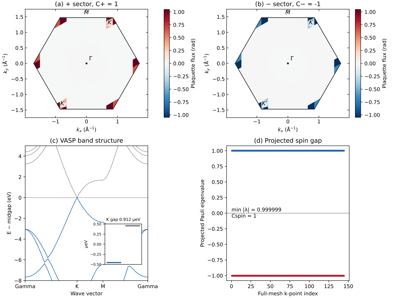
Figure 9. (a,b) Native positive- and negative-spin-sector plaquette fluxes on the 12 \times 12 mesh, shown without interpolation. The sectors carry opposite Chern numbers while the charge sum vanishes. (c) Actual VASP bands on \Gamma -K-M- \Gamma ; the inset resolves the 0.912 \text{ } \mu\text{eV} K-point gap using full-precision WAVECAR energies. (d) The projected-Pauli spectrum remains separated from zero. Mesh agreement establishes the integer result for this fixed input; the maps do not resolve the microscopic width or peak height of the Dirac curvature. Saved data and drawing commands reproduce all four panels.
