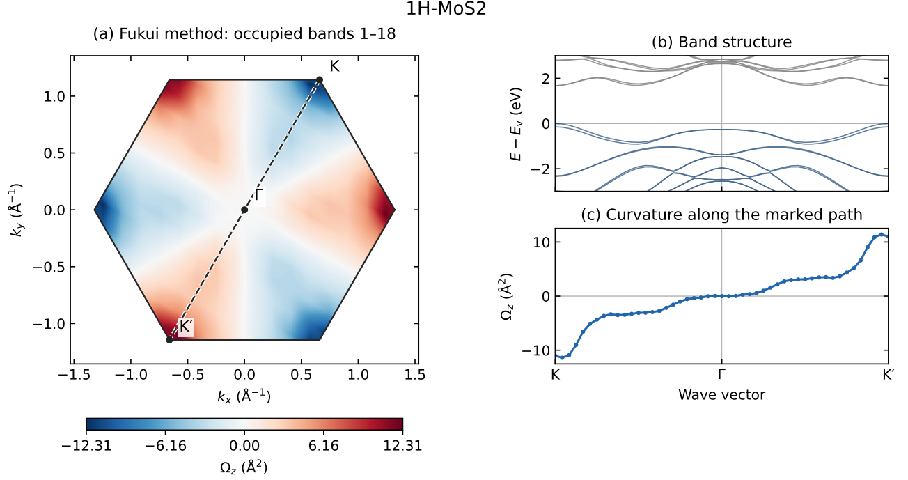
Figure 1. (a) Area-averaged Berry curvature from the Fukui method of occupied bands 1–18 in the Cartesian first Brillouin zone. The dashed line marks K – \Gamma – K' , with K = (1/3, 2/3) and K' = -K in reciprocal coordinates. Native 12 \times 12 plaquette values are displayed with periodic bilinear interpolation onto a 401 \times 401 Cartesian grid. (b) VASP band structure along that path; energies are relative to the valence-band maximum, with occupied bands in blue and empty bands in gray. (c) A periodic bilinear cut of the plaquette field along the marked path. This line visualizes panel (a), rather than adding an independent pointwise curvature calculation. Both right-hand panels share the same Cartesian path distance.
