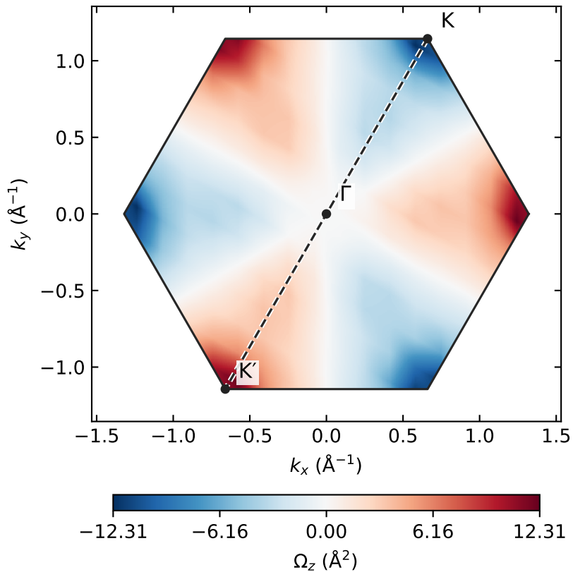
(a) Fukui method: occupied bands 1-18
