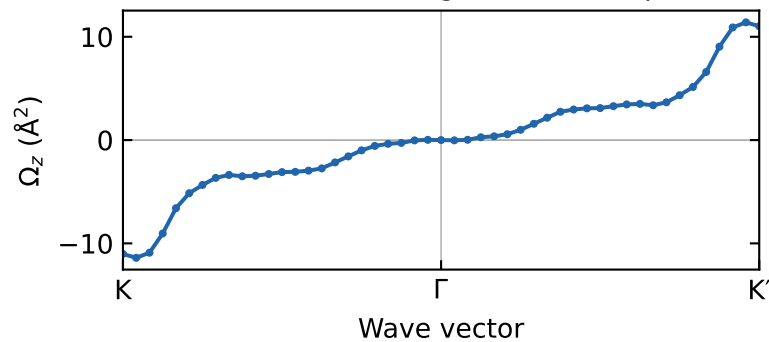
(c) Curvature along the marked path
