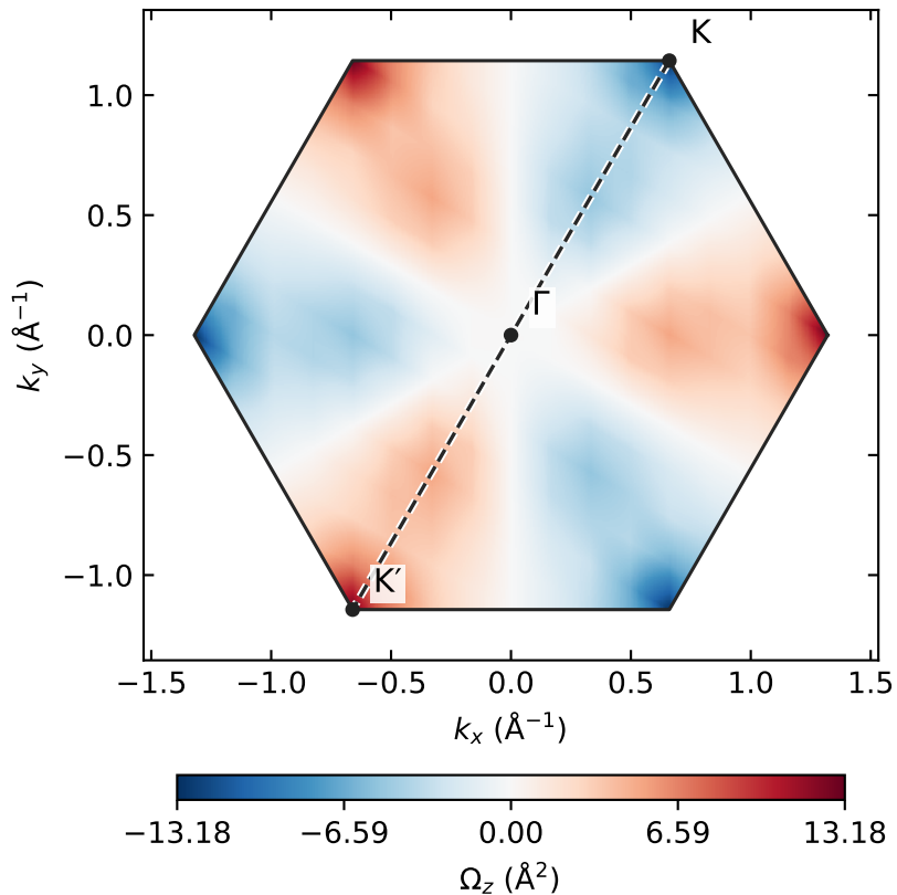
(a) Kubo formula: occupied bands 1-18
