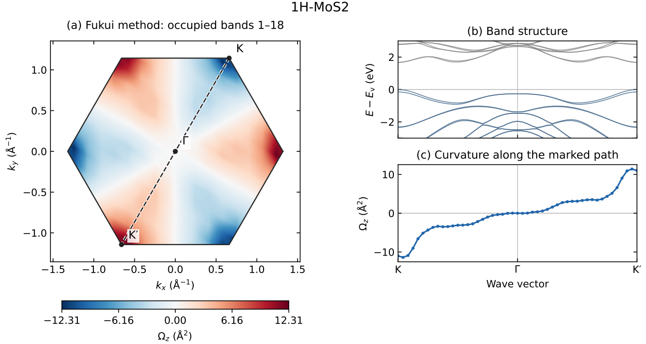
Figure 1. (a) Area-averaged Berry curvature from the Fukui method of occupied bands 1–18 in the Cartesian first Brillouin zone. The dashed line marks K– \Gamma –K', with K = (1/3, 2/3) and K' = -K in reciprocal coordinates. Native 12 \times 12 plaquette values are displayed with periodic bilinear interpolation onto a 401 \times 401 Cartesian grid. (b) VASP band structure along that path; energies are relative to the valence-band maximum, with occupied bands in blue and empty bands in gray. (c) A periodic bilinear cut of the plaquette field along the marked path. This line visualizes panel (a), rather than adding an independent pointwise curvature calculation. Both right-hand panels share the same Cartesian path distance.
