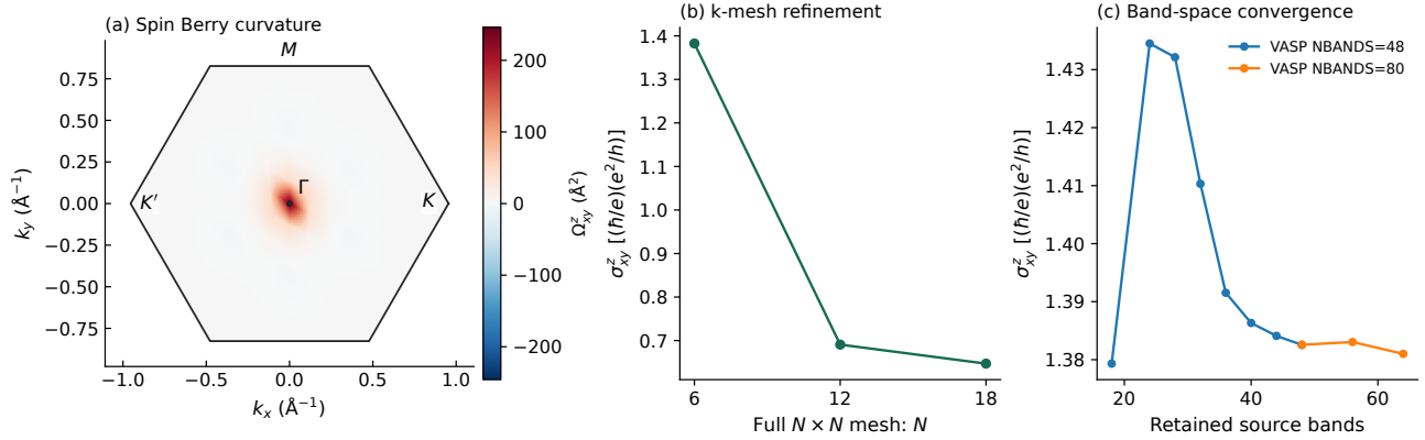
Figure 14. (a) Occupied-bundle spin Berry curvature \Omega_{xy}^z from PAW spin and full velocity matrices on the 12×12 VASP mesh, shown in the Cartesian first BZ. Periodic bilinear interpolation is used only for the color map. (b) Mesh refinement retaining 48 bands from 64-band VASP sources. (c) Retained-band studies from 48- and 80-band VASP sources at a fixed 6×6 mesh. The numerical integrals always use the original k points and weights.
