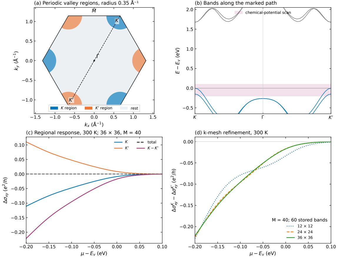
Figure 4. (a) Cartesian first BZ with periodic K/K' disks of radius 0.35 Å -1 and the marked K- \Gamma -K' line. (b) The matching 26-band VASP dispersion, with the chemical-potential interval shaded. (c) Regional Hall changes at 300 K on the 36×36 mesh, using 60 stored bands and pairs within bands 1–40. (d) Mesh refinement at that fixed band window. Energies are relative to each source's valence-band maximum; the band path uses the same density and cutoff.
