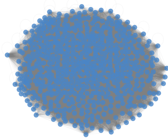
100 Neighbors
