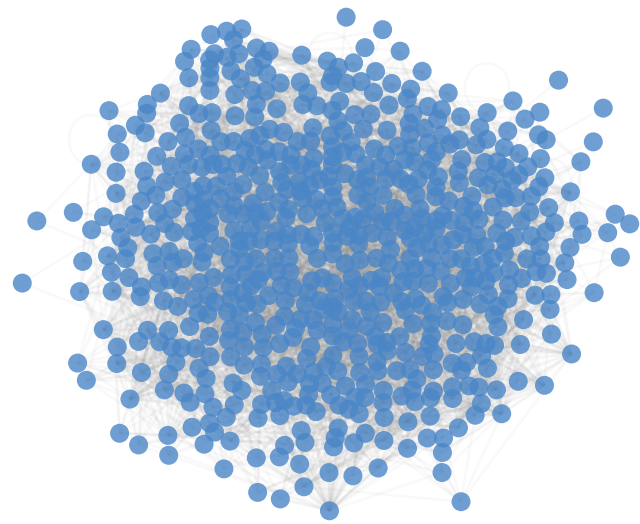
50 Neighbors
