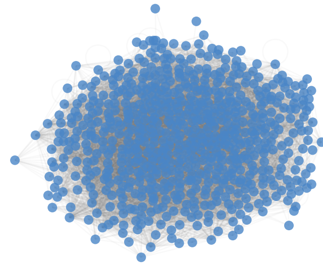
200 Neighbors
