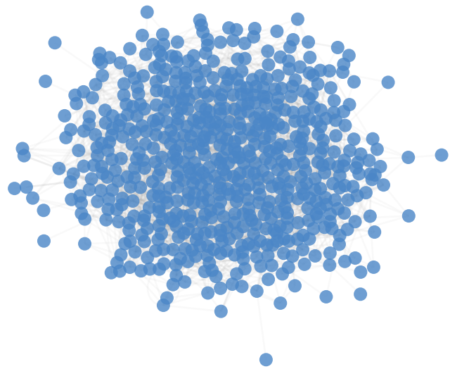
30 Neighbors
