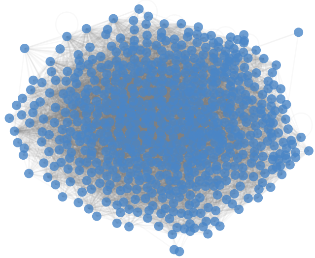
25 Neighbors
