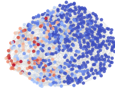
Coag Rate
