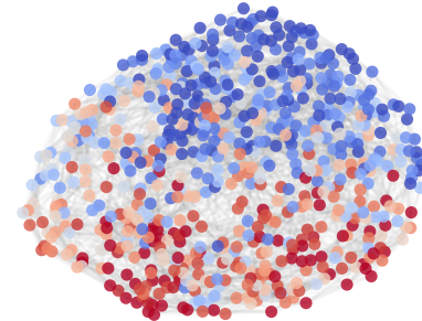
Renal Rate
