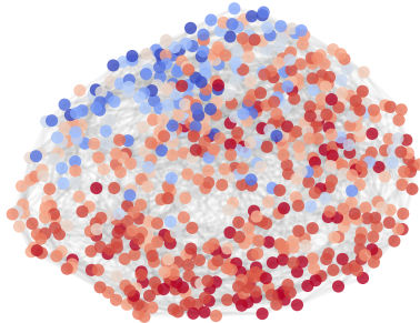
Resp Rate
