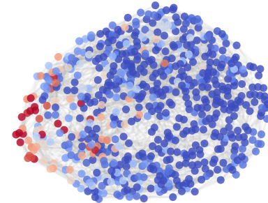
Liver Rate
