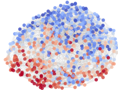
Cardio Rate
