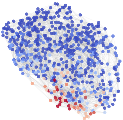
Liver Rate
