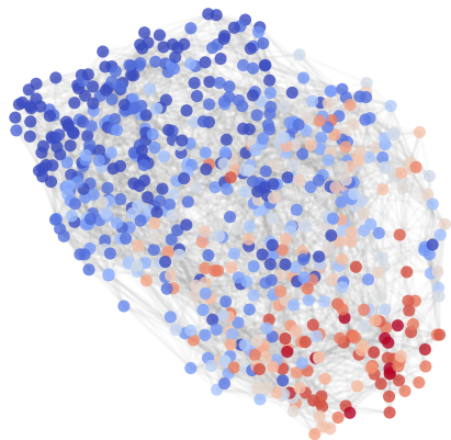
Renal Rate
