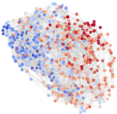
Resp Rate
