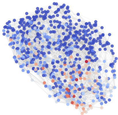
Coag Rate
