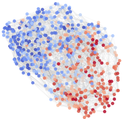
Cardio Rate
