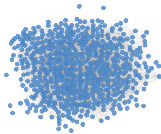
50 Neighbors
