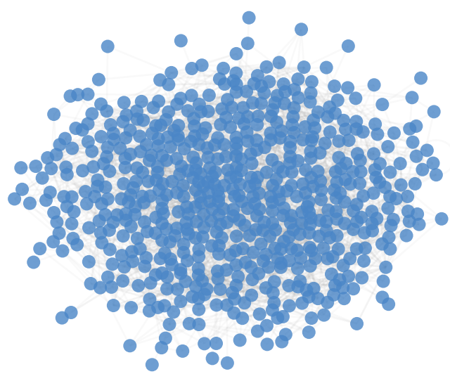
30 Neighbors
