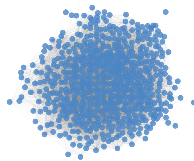
100 Neighbors
