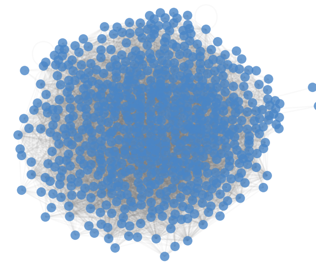
200 Neighbors
