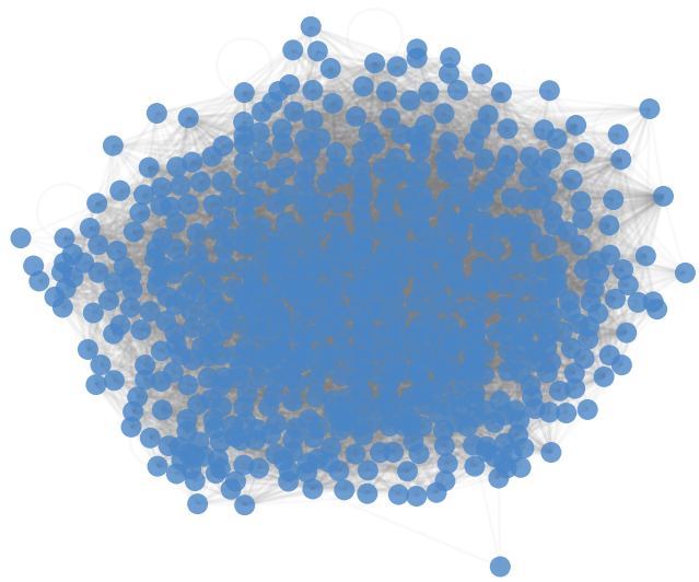
25 Neighbors
