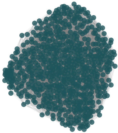
50 Neighbors
