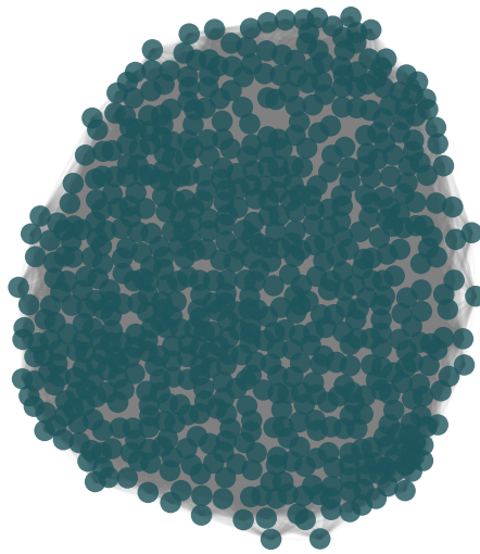
100 Neighbors
