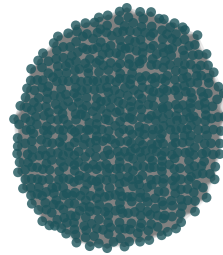
500 Neighbors
