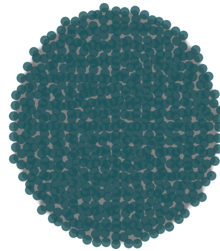
600 Neighbors
