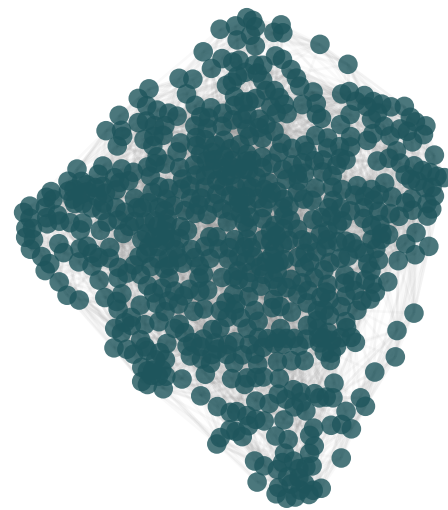
300 Neighbors
