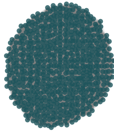
400 Neighbors
