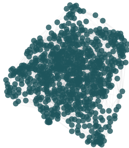
200 Neighbors
