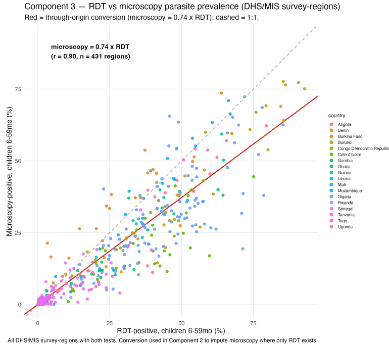
Figure 5: Component 3: RDT vs microscopy
