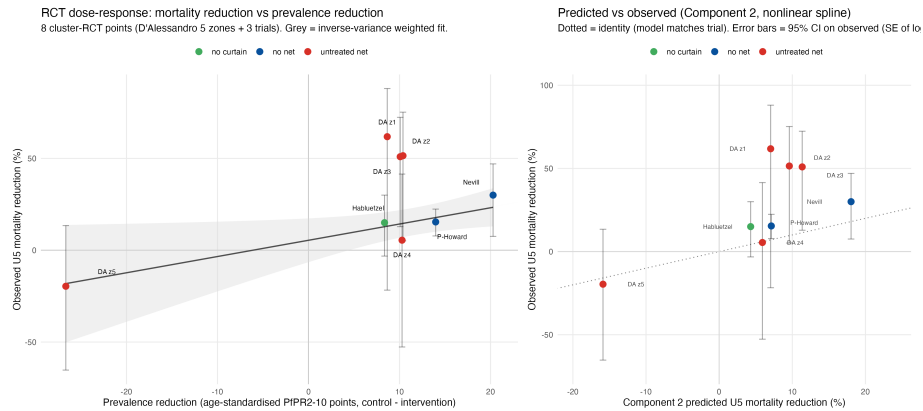
Figure 9: RCT triangulation: dose-response and Component 2 predicted vs observed
