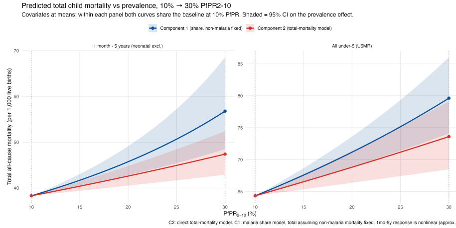
Figure 6: Predicted total child mortality vs prevalence, 10% to 30% PfPR2-10
