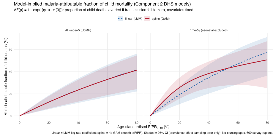
Figure 7: Malaria-attributable fraction of child deaths vs PfPR2-10
