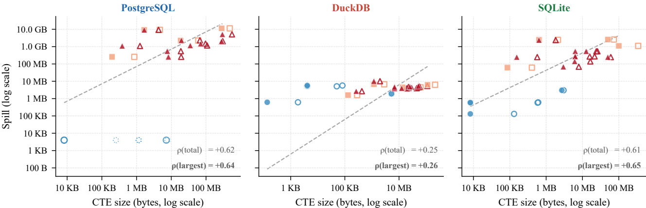
Spill vs CTE size (log-log) — filled = largest CTE, open = total CTE (bolder \rho = stronger predictor)
