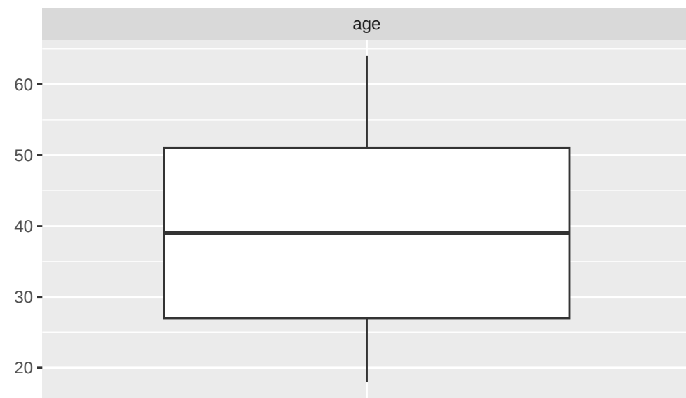
Boxplots of the numeric data
