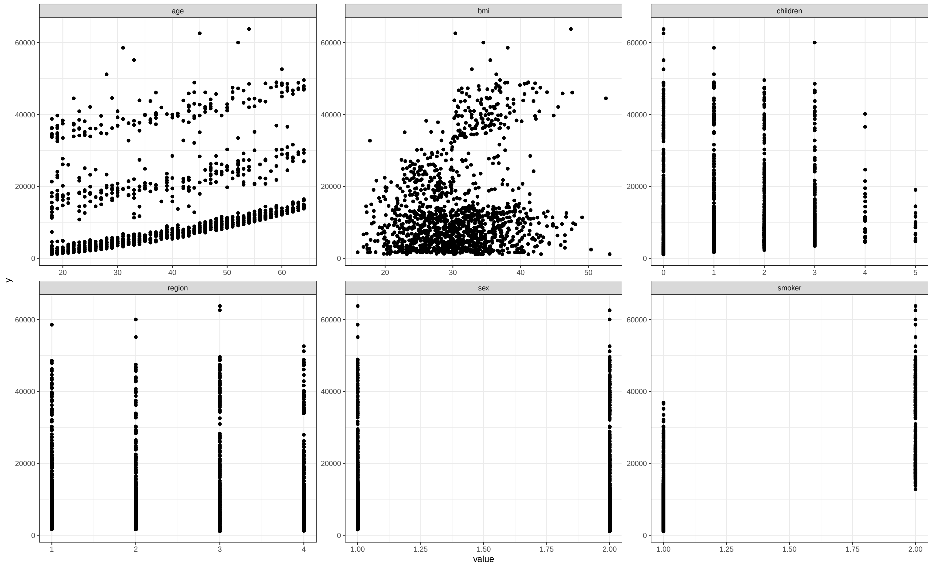
y (predictor variable) vs target variables
