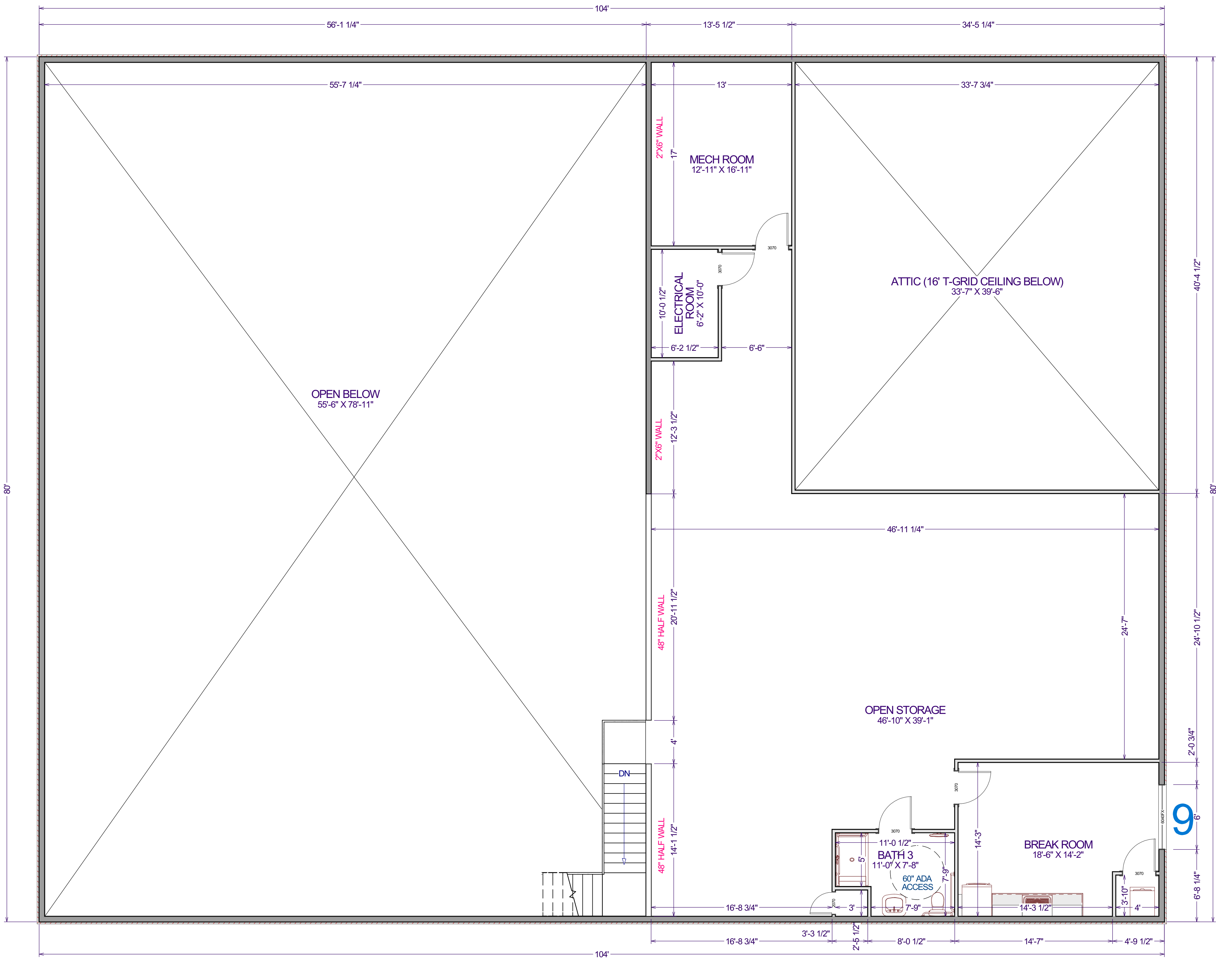
FLOOR PLAN - 2ND 3/16"= 1'
