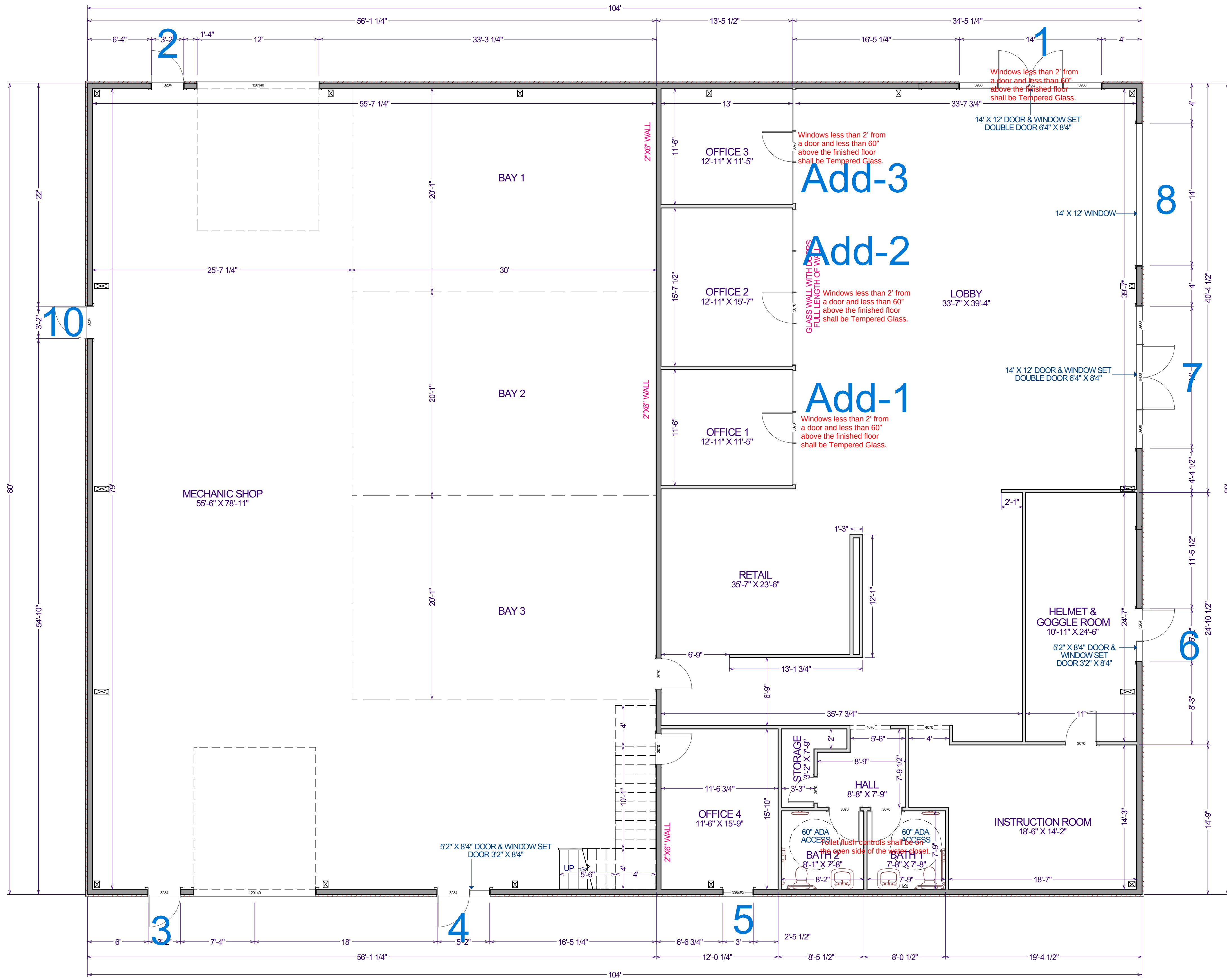
FLOOR PLAN - 1ST 3/16"= 1'
