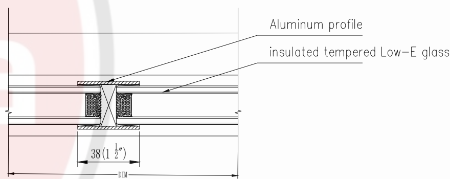
Butted Structural Joint(Scale:20:1)
