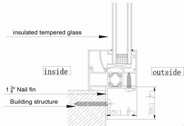
1 3/8" Nail Fins
