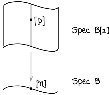
FIGURE 13.4. The geometry behind the proof of Proposition 13.3.7.
