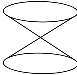
FIGURE 9.4. The cone x^2 + y^2 = z^2 in \mathbb{A}^3 .
