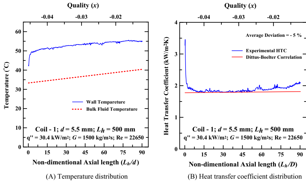
Fig. 3. Temperature and heat transfer coefficient distribution in single phase flow along the axial length of tube.
