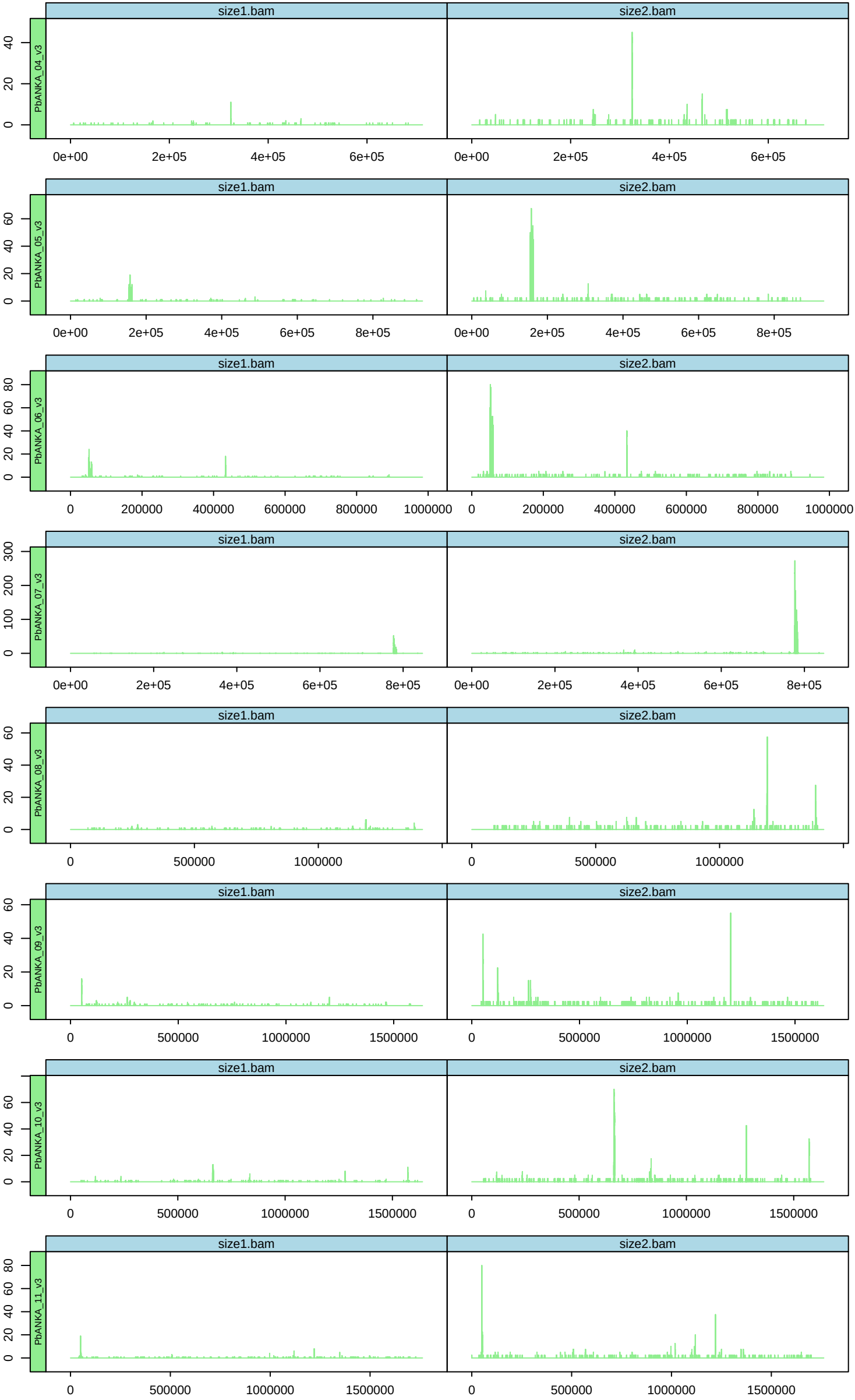
Coverage depths
