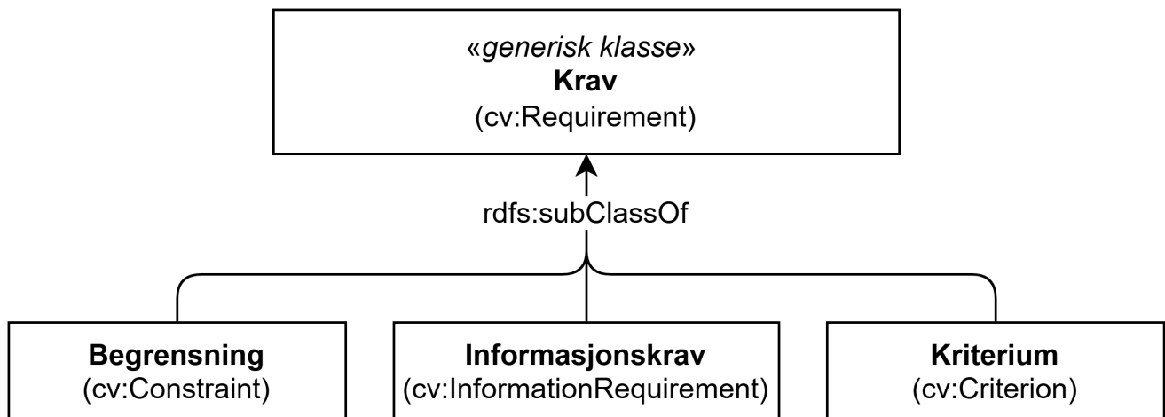
Figur 9. Klassen Krav (cv:Requirement).
