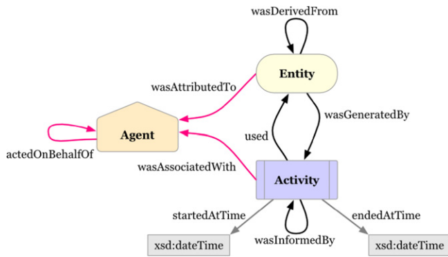
Fig. 1. The core concepts of PROV. Source: Taken from [14].
