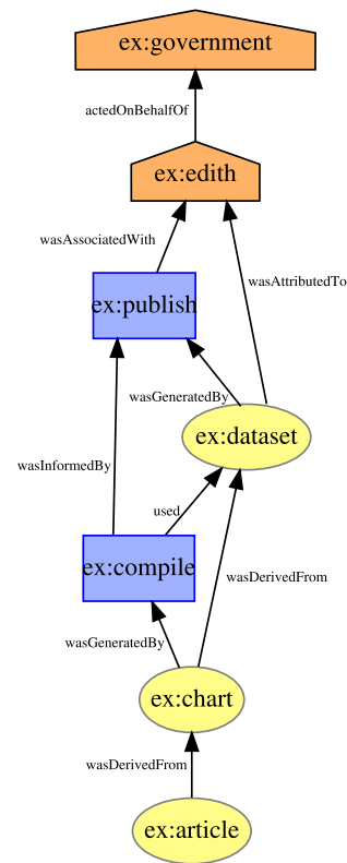
Fig. 2. Example PROV graph (turtle file ‘Inline Supplementary Computer Code S1’ and PROV-N file ‘Inline Supplementary Computer Code S2’ are available online at http://dx.doi.org/10.1016/j.websem.2015.04.001 ).
