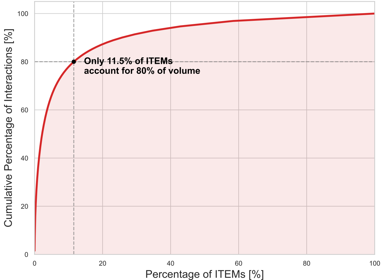
Cumulative Item Popularity (Pareto Principle)
