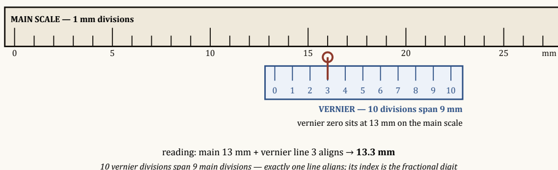
Figure 20.1. The vernier trick: 10 vernier divisions span 9 main divisions, so exactly one vernier line aligns — its index is the fractional digit. Ten minutes of practice replaces a magnifier and a guess.
