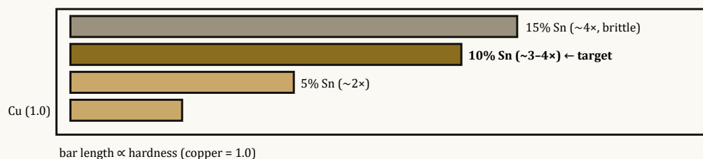
Fig 10.2 — Why ~10% tin (relative hardness, copper = 1.0)
