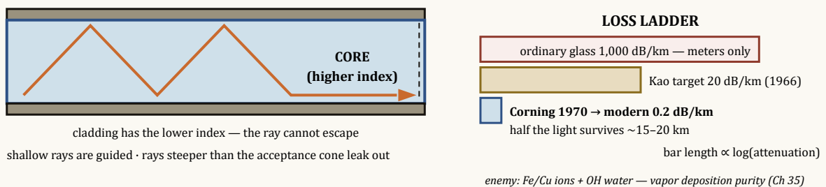
Fig 41.1 — Trap light by index step; win by purity (dB/km)
