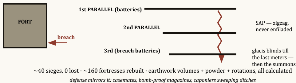
Figure 48.2. Parallels trench across the front (batteries each step), zigzag saps crawl forward immune to enfilade, breach batteries open the wall — then the courteous surrender letter. Siegecraft as scheduled engineering: volumes, powder, reliefs, all tabulated.
