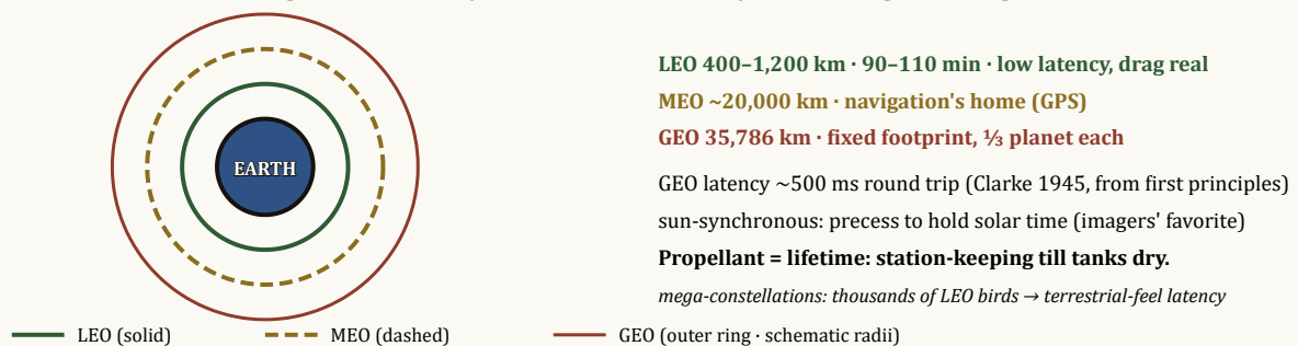
Fig 40.1 — Pick your altitude: latency vs coverage vs drag
