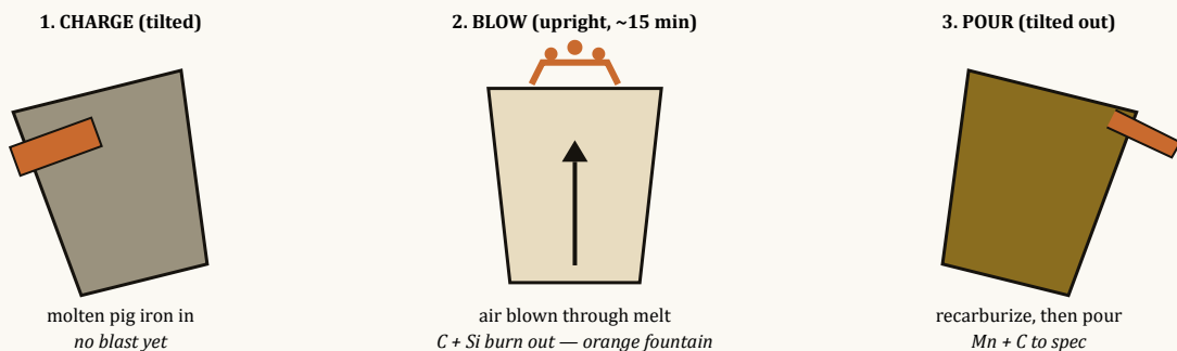
Fig 27.1 — Bessemer blow in three tilts (side view)
