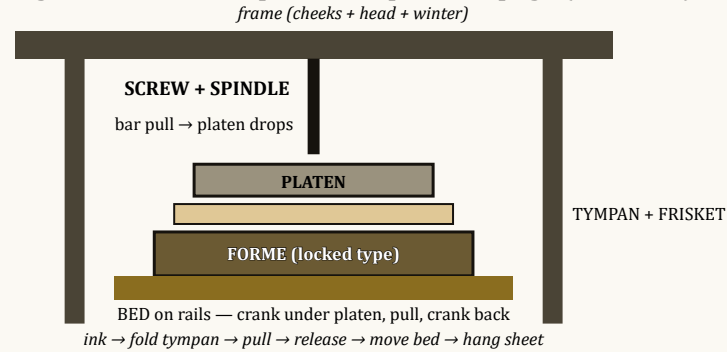
Fig 18.2 — Common press: one pull, one page (side view)
