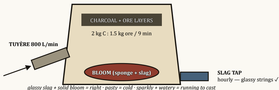
Fig 14.1 — Bloomery: solid iron, fluid slag, never molten
