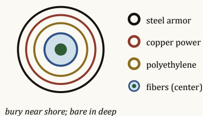
Figure 41.2. Left: concentric survival — fibers ride the neutral center, copper feeds repeaters, steel takes the bites. Right: colors multiply capacity — one fiber carries a rainbow, amplifiers boost light without ever decoding it.
