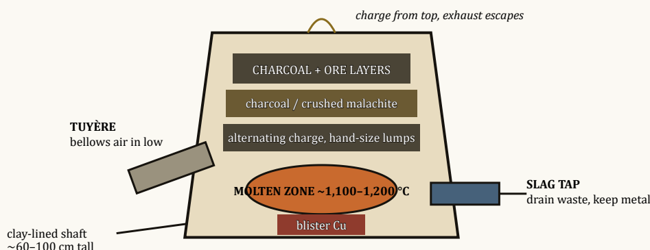
Fig 10.1 — Clay shaft furnace for copper smelting (cross-section)
