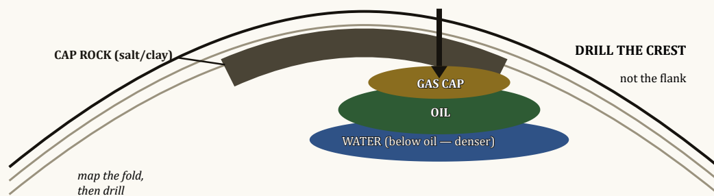
Fig 28.1 — The anticline trap: why oil sits where it sits
