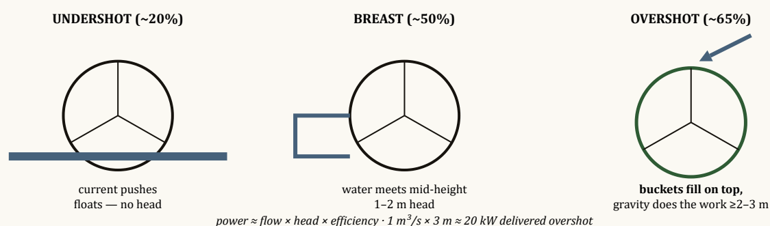
Fig 16.1 — Head decides the wheel (efficiency in brackets)
